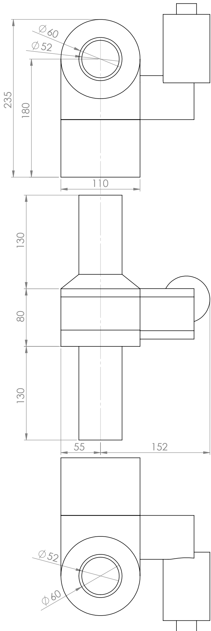
ROTOR RAU\HR Dimmension: mm
