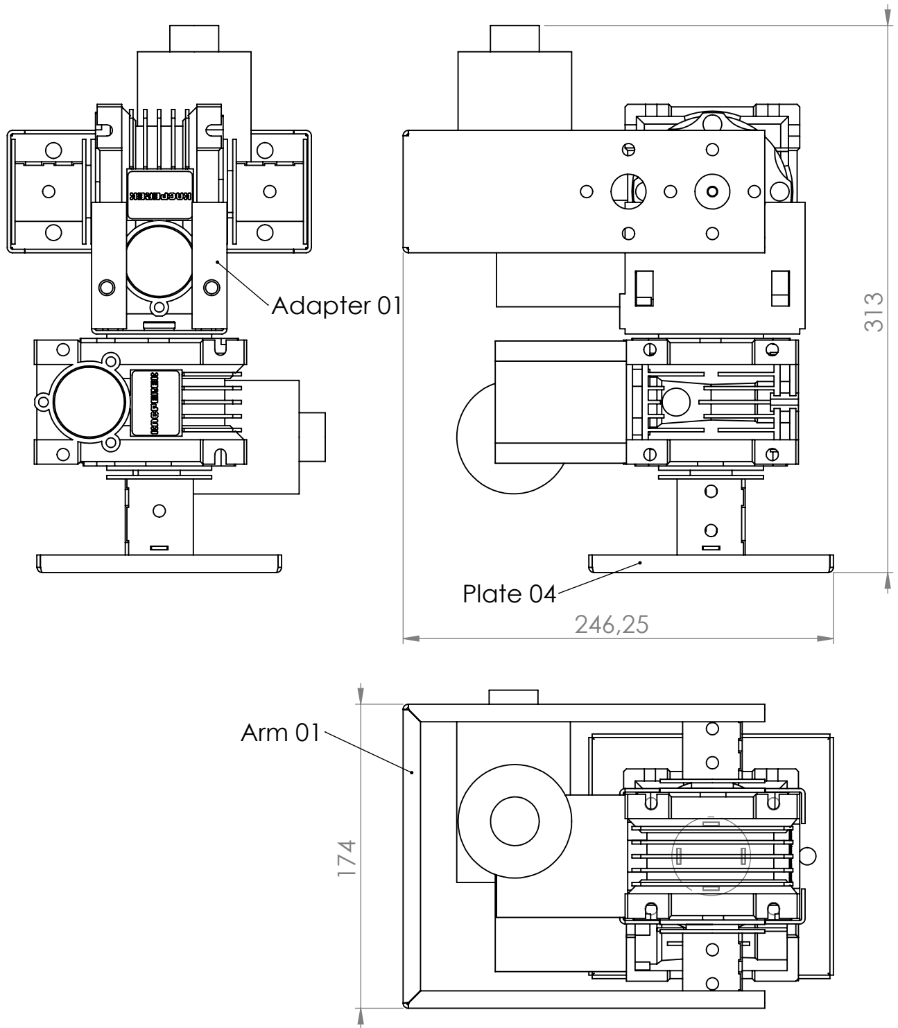
ROTOR SPX AZ\EL-01 Dimmension: mm
